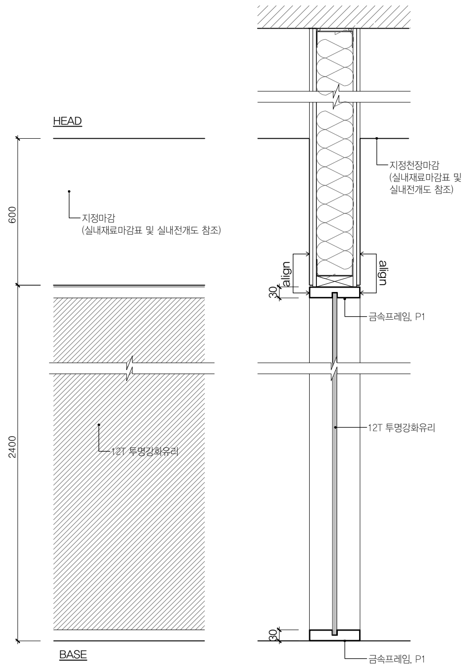
01 TYPE 4 SCALE 1:10
