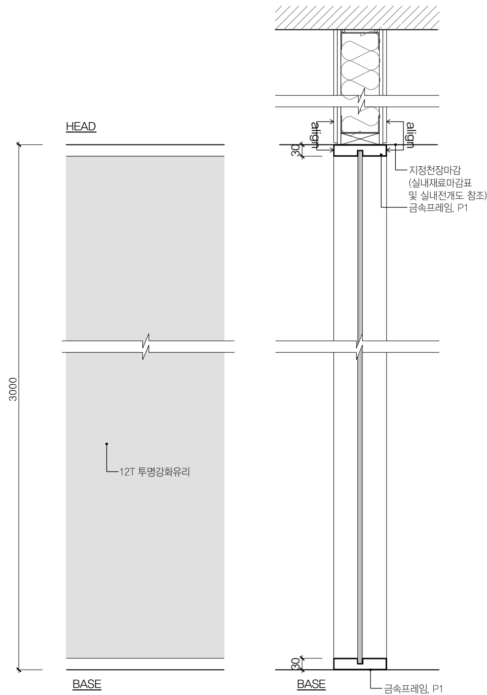
02 TYPE 6 SCALE 1:10
